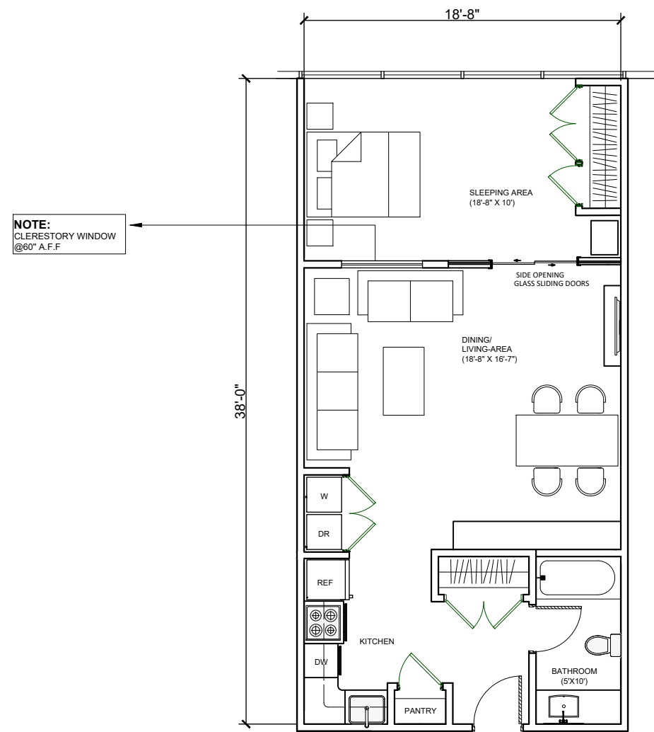
OPTION 2 AREA=718 SQ FT
