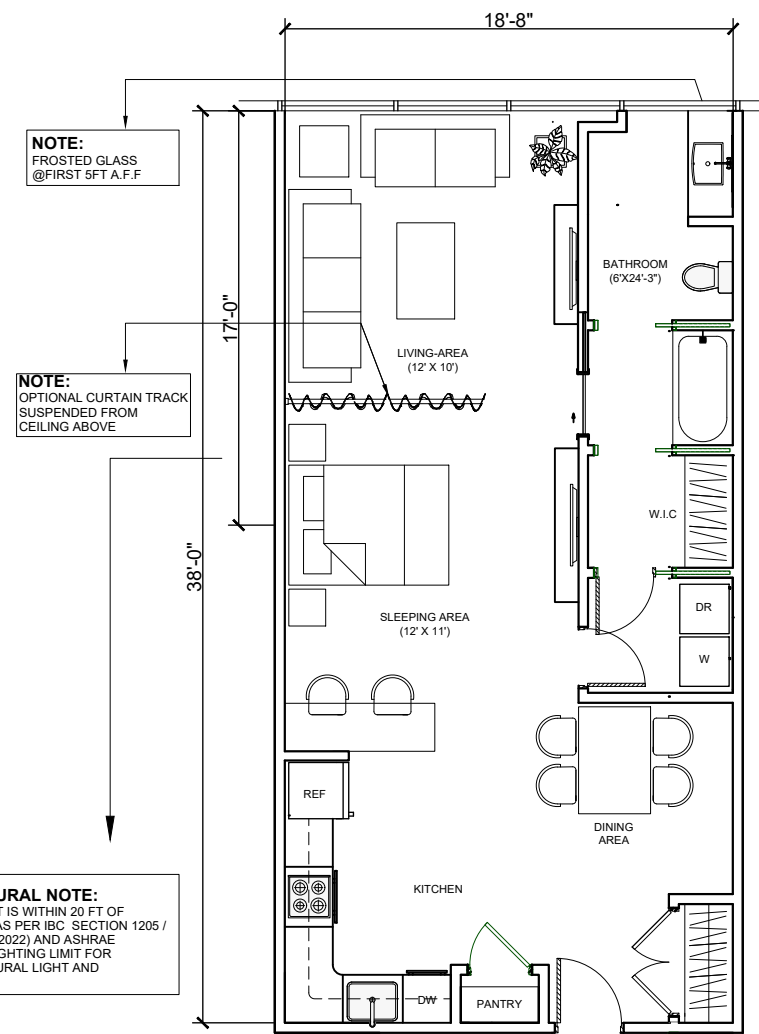
OPTION 3 AREA=718 SQ FT
