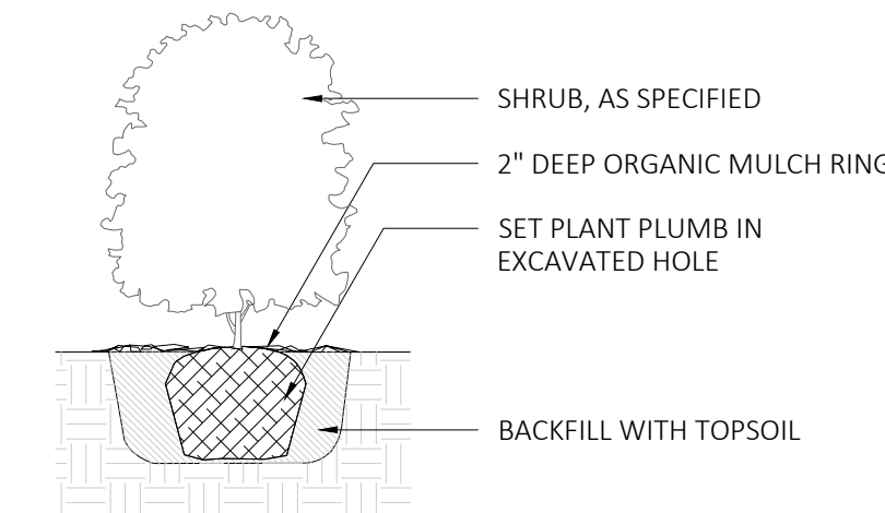
1 SHRUB & ORNAMENTAL GRASS PLANTING SCALE: 1/2" = 1'
