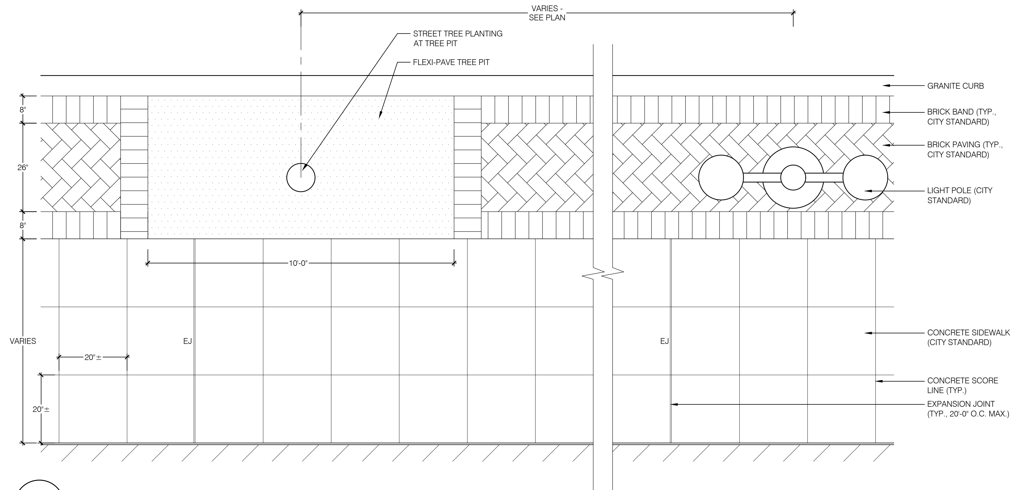
5 TYPICAL SIDEWALK PLAN
