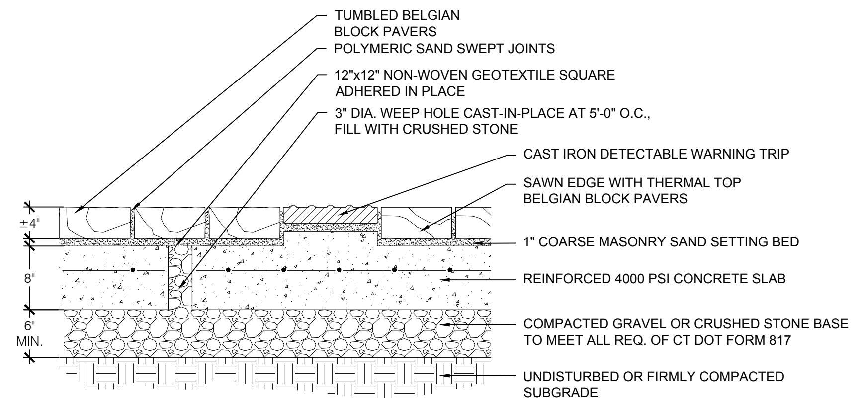
1 BELGIAN BLOCK DETAIL
