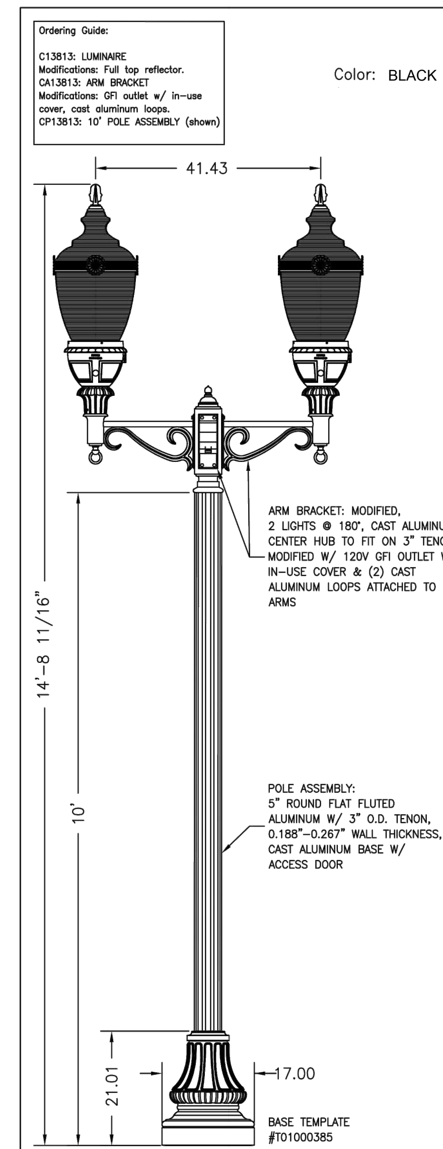
6 DOUBLE LUMINAIRE LIGHT POLE (CITY STANDARD) SPL-2.0
