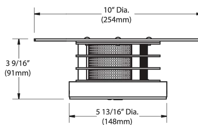
8 DECORATIVE LIGHT FIXTURE MOUNTED TO GREENSCREEN SPL-2.1
