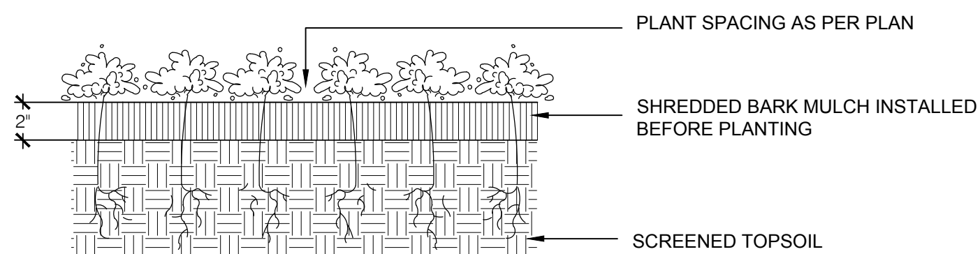
1 GROUNDCOVER / PERENNIAL PLANTING SPL-2.1
