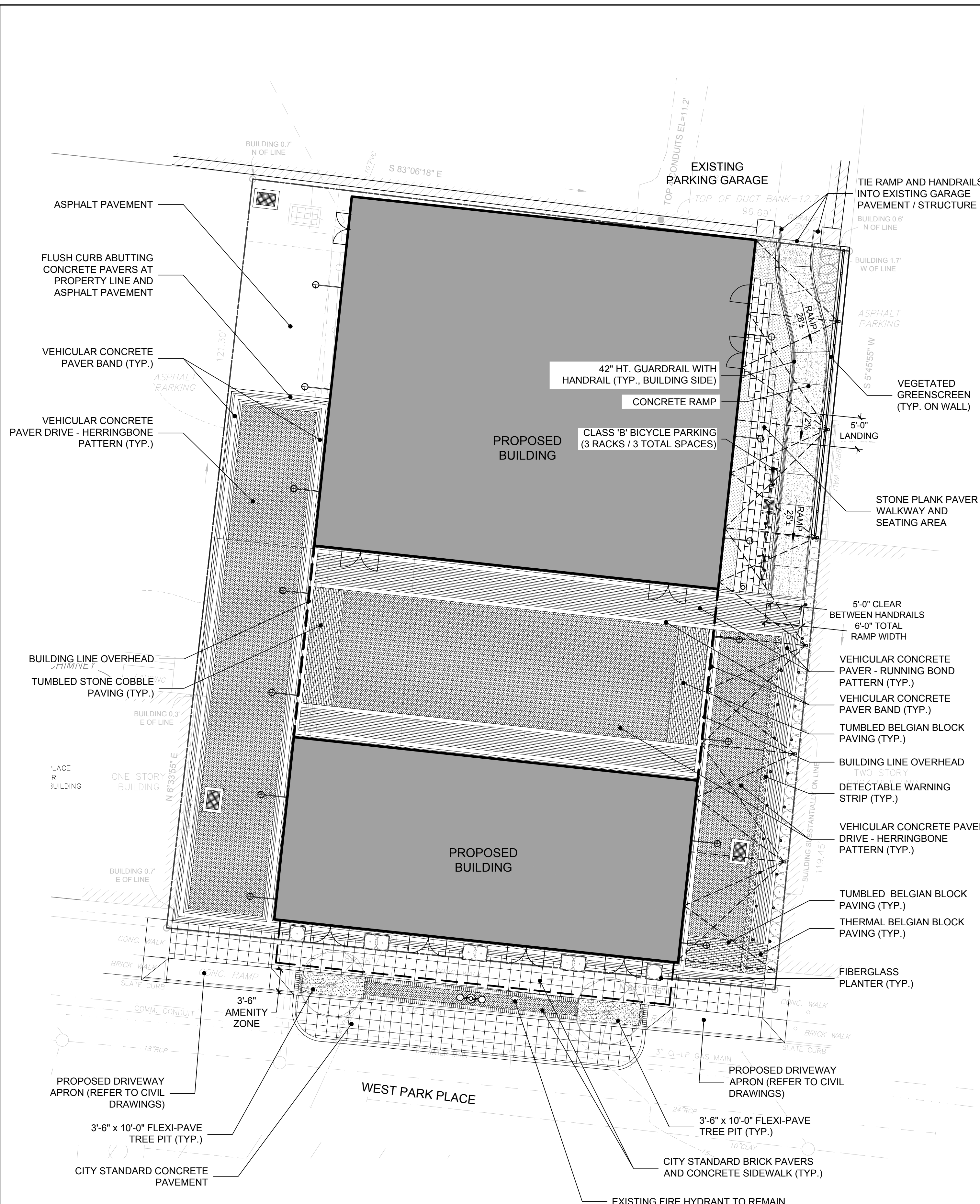
1 LANDSCAPE SITE MATERIALS AND LAYOUT PLAN SPL-1.0
