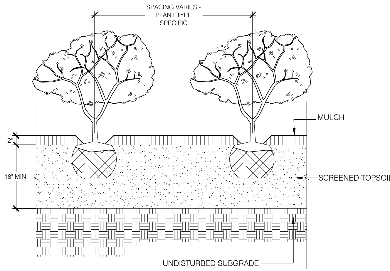
3 SHRUB PLANTING SPL-2.1
