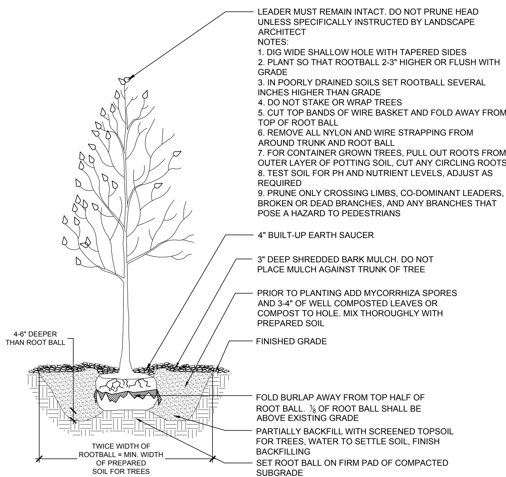
2 TREE PLANTING - TYPICAL SPL-2.1
