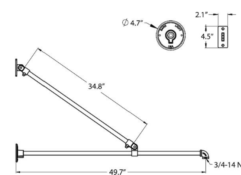
7 BUILDING MOUNTED GOOSENECK LIGHT SPL-2.0
