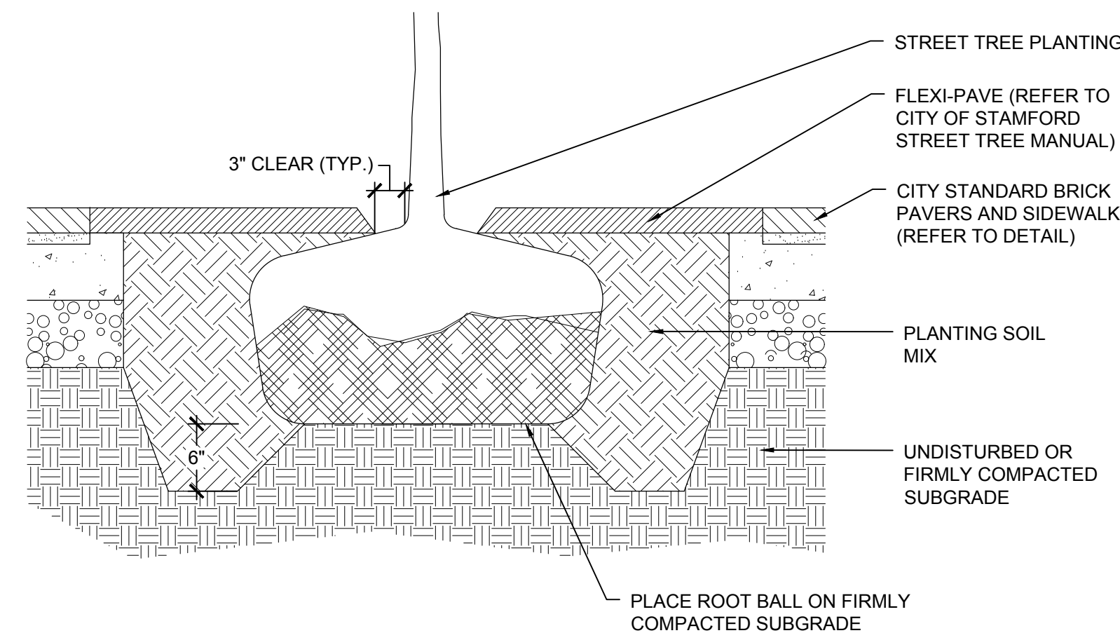
2 FLEXI-PAVE TREE PIT
