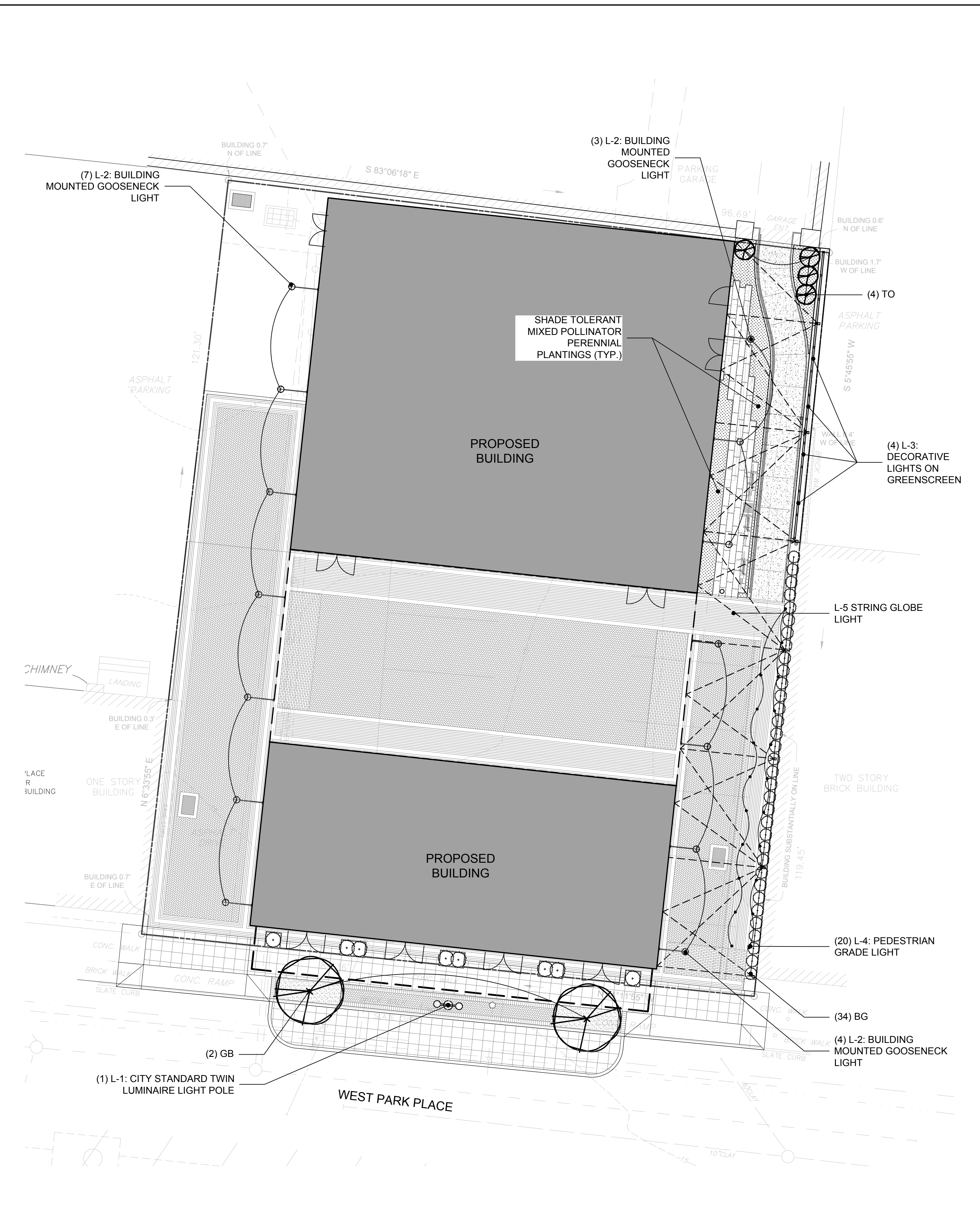
2 SITE PLANTING AND LIGHTING PLAN SPL-1.0
